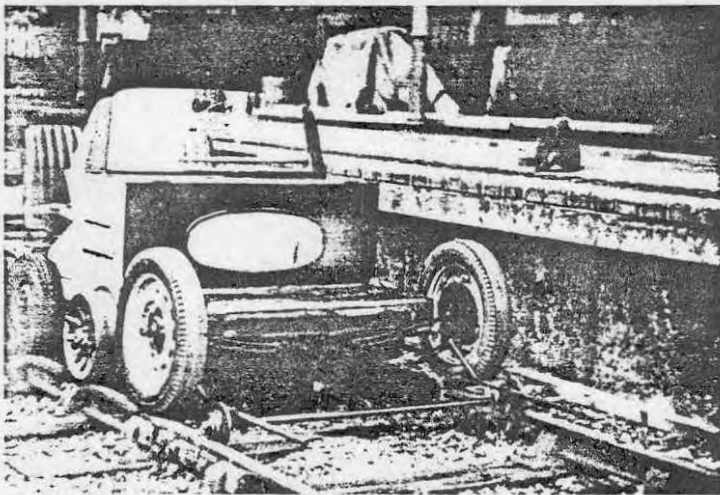
Pneumatic tyred road/rail transport proposed in the Lucas corporate plan. On the test vehicle flanged wheels provide guidance, but the vehicle is steered by tread forces.
